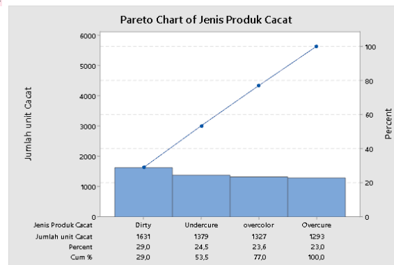
Gambar 4. Diagram Pareto
