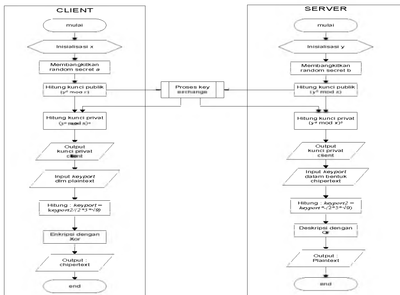
Gambar 2 Flowchart Algoritma AA
