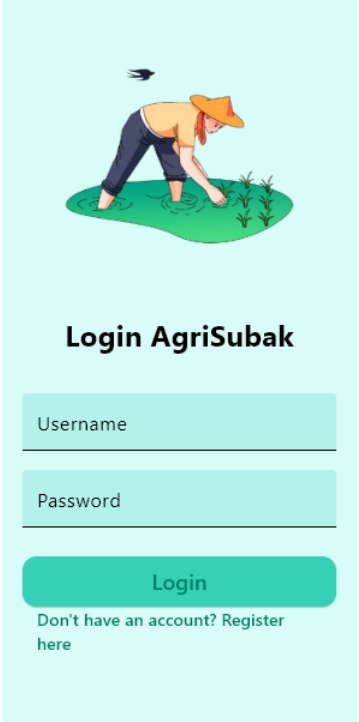
Figure 7. Login Page
