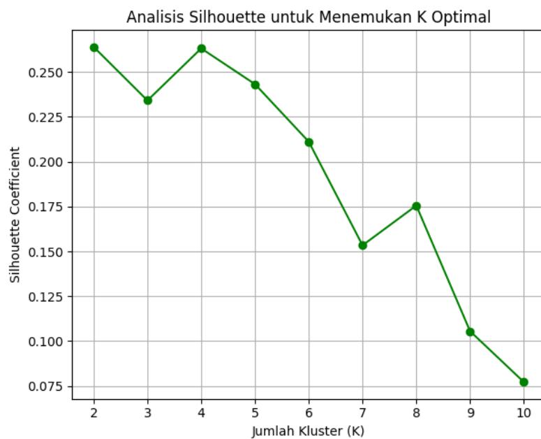
Figure 3. Silhouette Analysis
