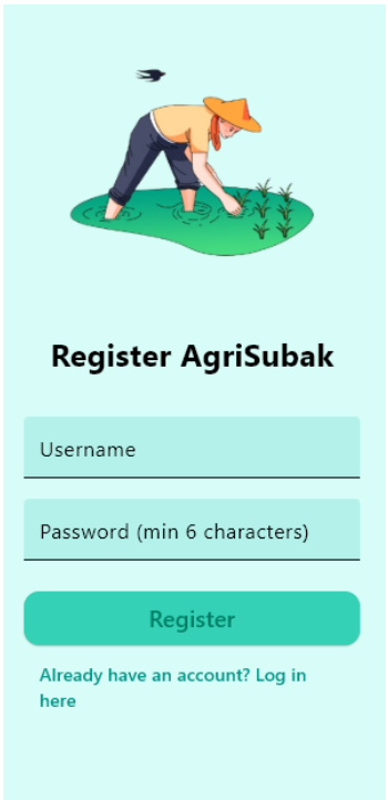
Figure 6. Registration Page
