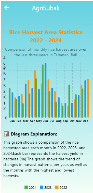
Figure 9. Statistics Page
