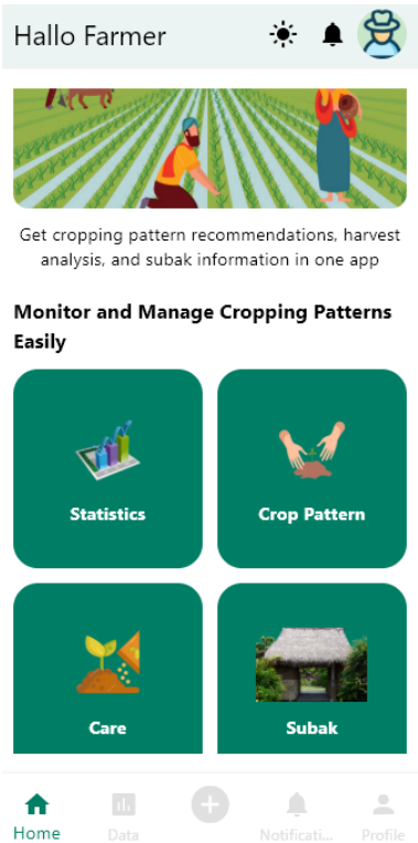
Figure 8. Dashboard Page
