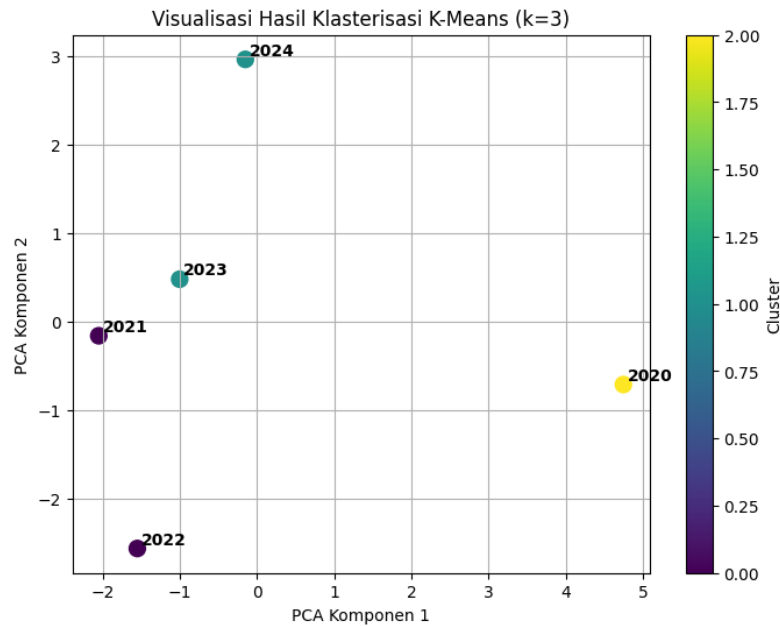
Figure 4. Visualization of K-Means Clustering Results, k=3
