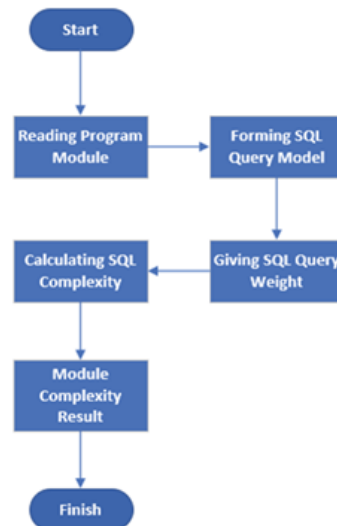
Figure 2. SQL Complexity Method [13]
