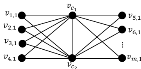
Figure 3. Graph B_{C_3,m}
