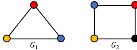
Figure 1. Vertex coloring.
