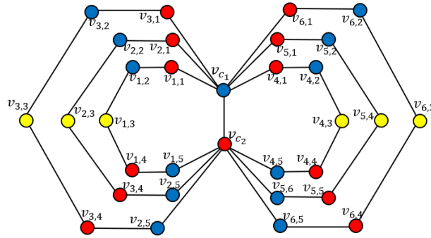
Figure 5. The chromatic number of the graph B_{C_7,6}
