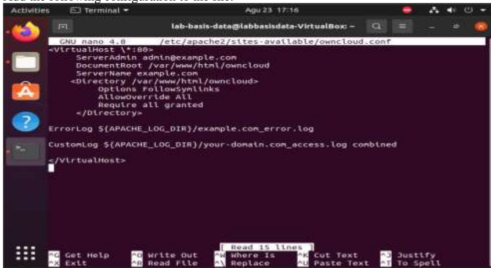
Figure 10. Addition of configuration to the file
