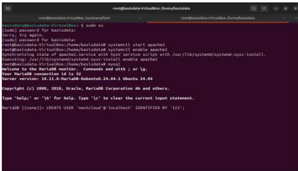
Figure 4. Creation of database and user for Nextcloud
