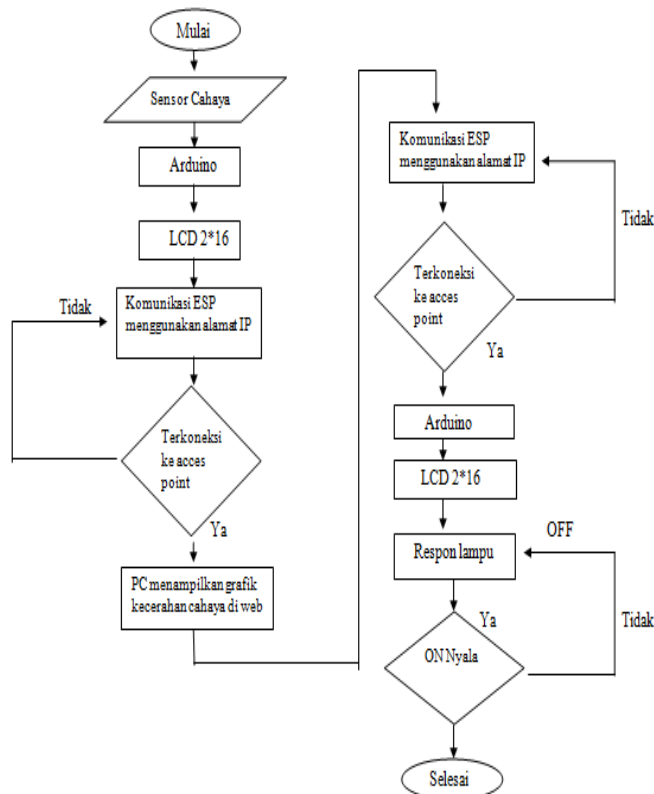
Gambar 3. Flowchart Sistem
