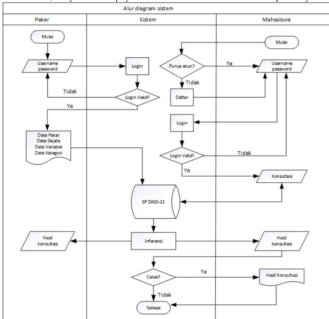
Figure 1. System Flowchart
