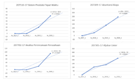
Figure 10. Prediction Graph
