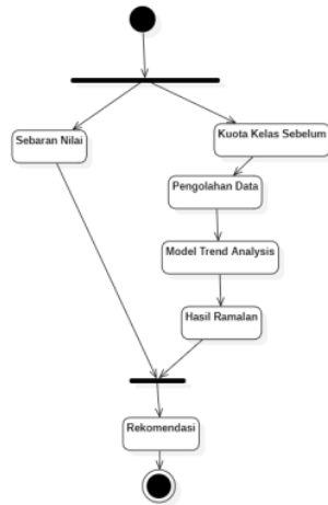
Figure 5. Activity diagrams
