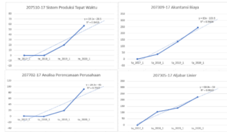
Figure 10. Prediction Graph
