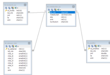
Figure 7. Table Relations
