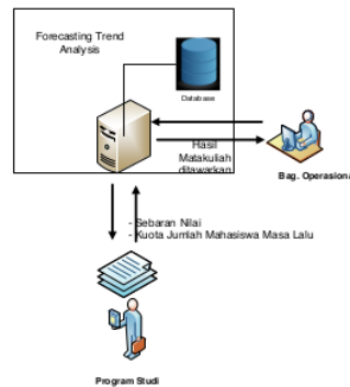
Figure 1. Program Architecture
