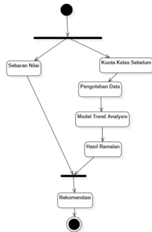
Figure 5. Activity diagrams
