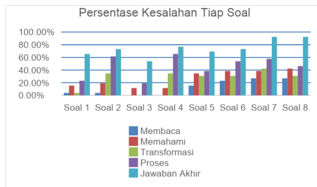
Gambar 1. Diagram persentase kesalahan tiap soal
