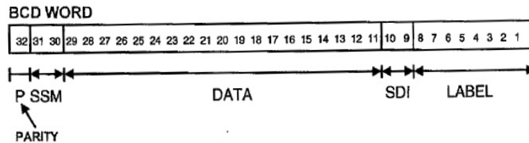
Gambar 4. BCD word format
