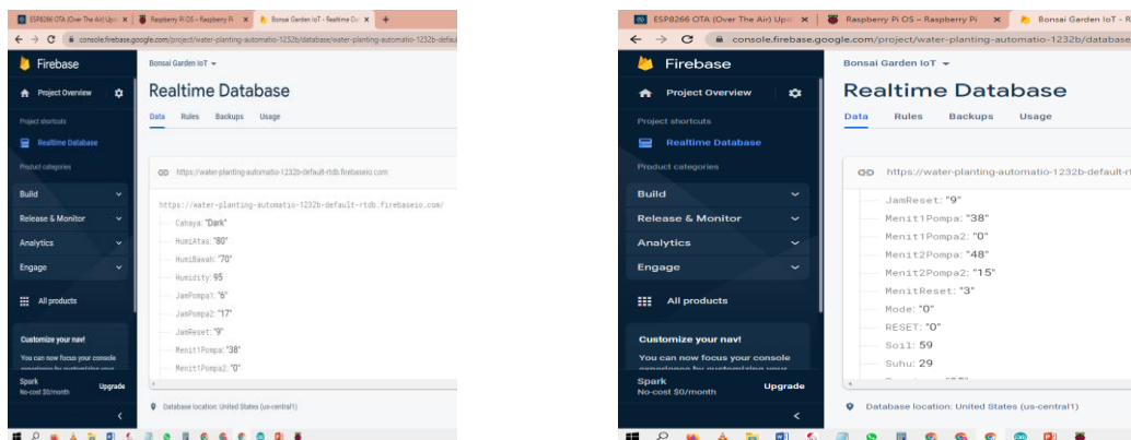
Gambar 12 Tampilan Firebase
