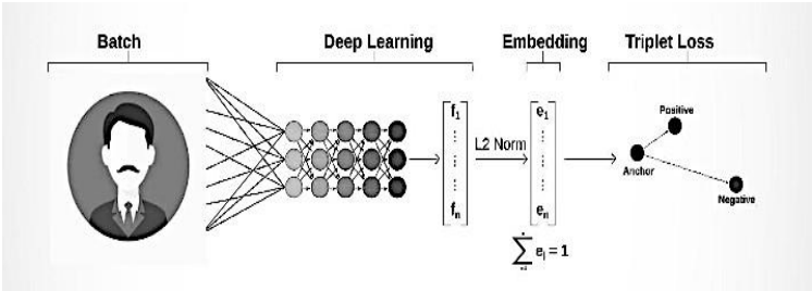
Figure 2. FaceNet Workflow
