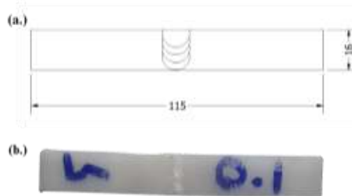
Gambar 12. Kupon Uji bending (a.) dimensi uji bending (b.) kupon pengujian
