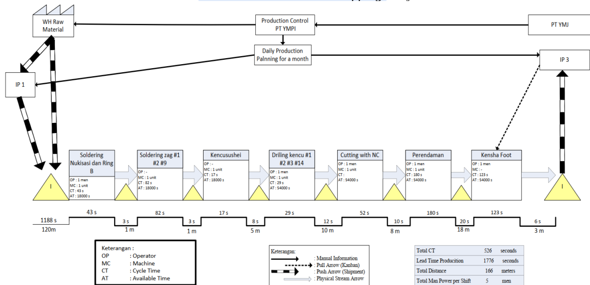
Gambar 2. Value Stream Mapping Body Flute
