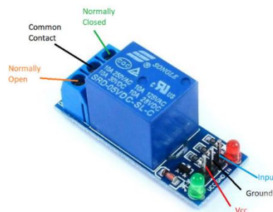
Gambar 5. Relay
