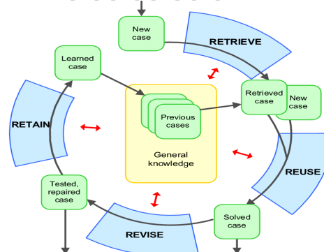
Gambar 1 Metode Case based reasoning [12]
