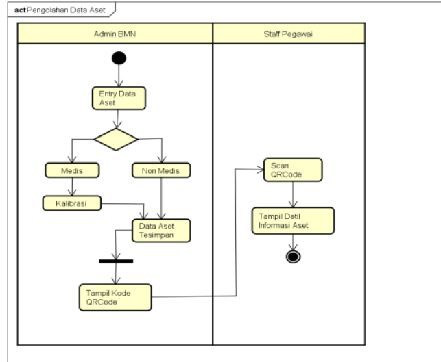
Gambar 4. Activity diagram pelaporan aset
